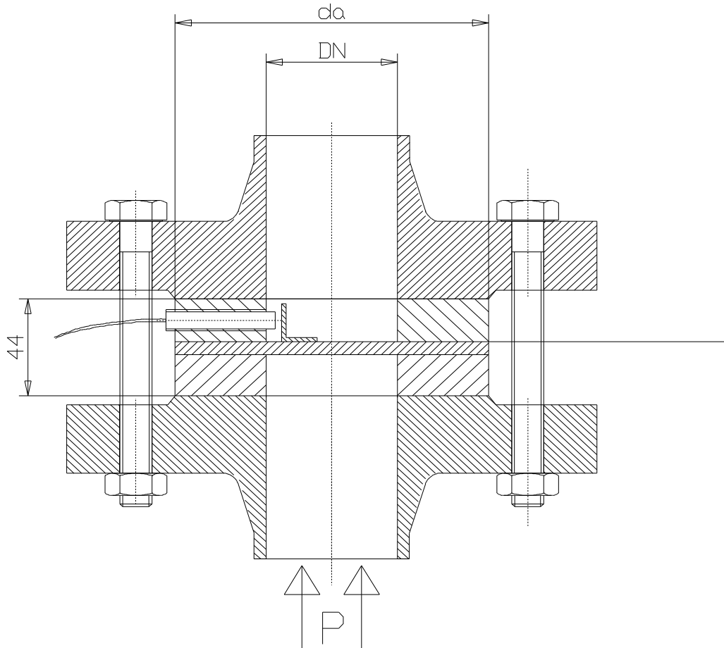
Dimensions "da" depends on DN and PN
