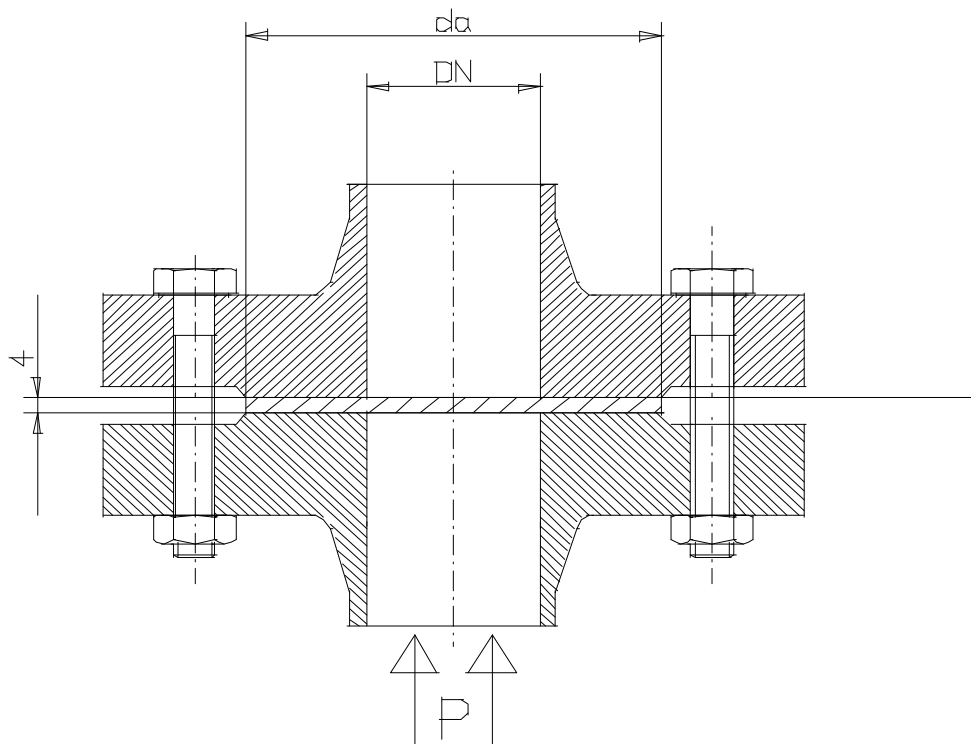
Dimension "da" depends on NPS and pressure rating of flange
